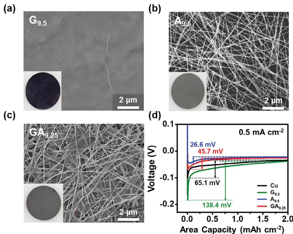
Figure 4. FE-SEM top-view images of a) G_{9.5} , b) A_{9.5} , and c) GA_{9.25} . The insets are optical photographs of each sample. d) Voltage-capacity profiles of Cu , G_{9.5} , A_{9.5} , and GA_{9.25} in 1 M LiTFSI in DOL/DME (1:1) electrolyte with 1 wt% LiNO_3 additives at 0.5 \text{ mA cm}^{-2} .
