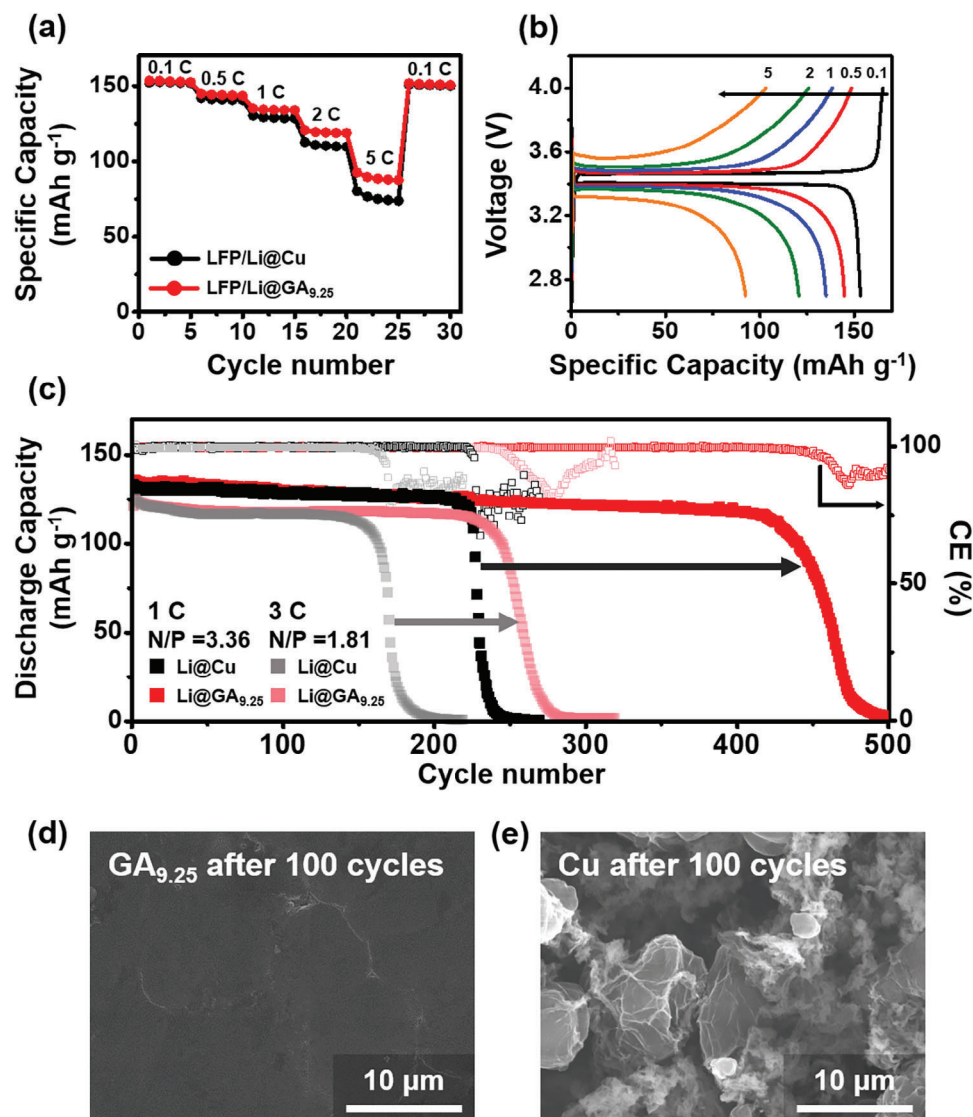
Figure 8. a) Rate performances of a full cell after Li plating with 2 mAh cm -2 at different current rates, ranging from 0.1 to 5 C, compared to LFP/Li@Cu and LFP/Li@GA 9.25 . b) Charge/discharge curves of LFP/Li@GA 9.25 full cell at various current rates. c) Cycle performance and Coulombic efficiency of LFP/Li@Cu and LFP/Li@GA 9.25 full cells after Li plating with capacities of 4 mAh cm -2 at 1 C and 2 mAh cm -2 at 3 C. FE-SEM images of the anode surfaces from the disassembly of d) LFP/Li@GA 9.25 and e) LFP/Li@Cu full cells after 100 cycles at 1 C. The pre-deposition of Li in the samples was 4 mAh cm -2 .
