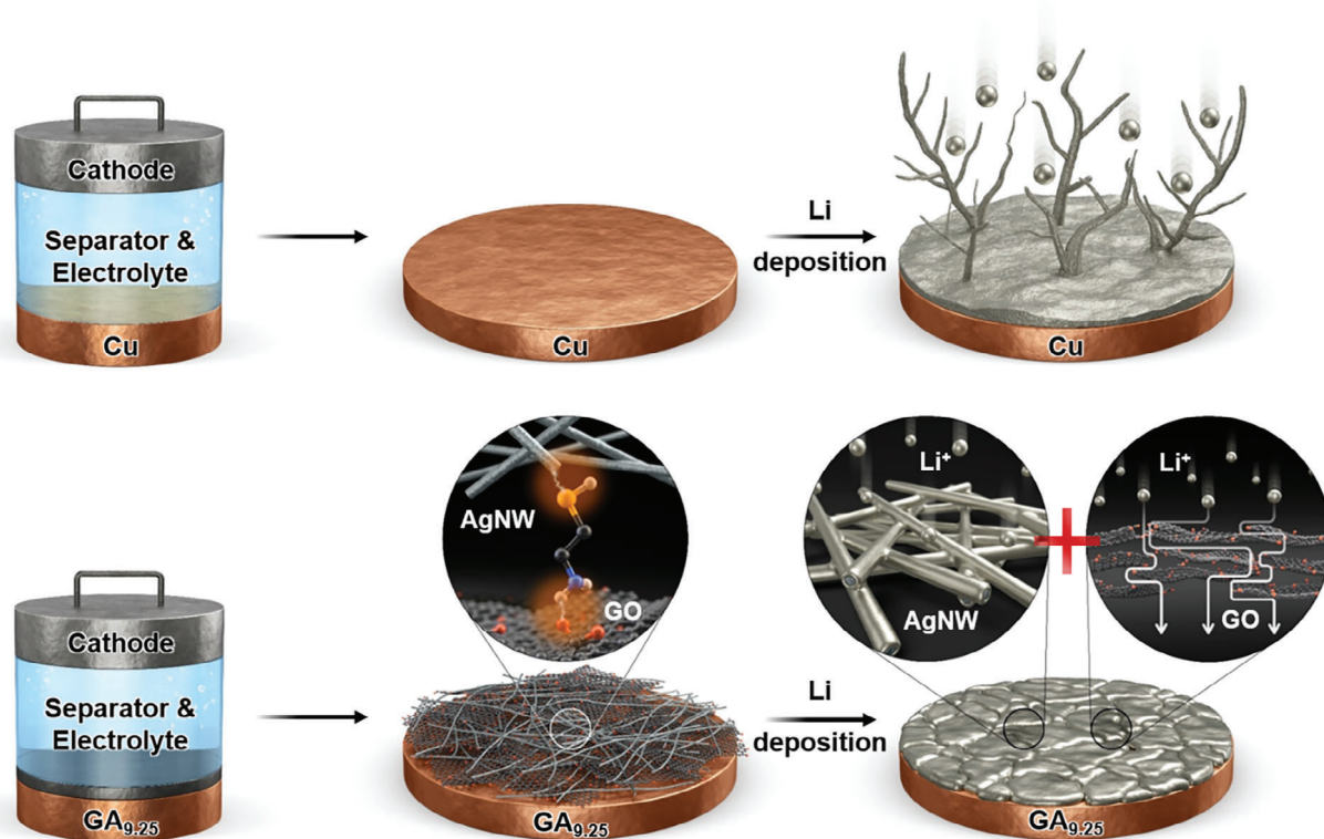
Figure 1. Schematic illustrating Li growth on bare Cu foil and the GO/AgNW LbL thin film-coated Cu foil. GA 9,25 refers to the (GO/MEA/AgNW/MEA) 9,25 LbL sample, which is the representative sample used in this study.
